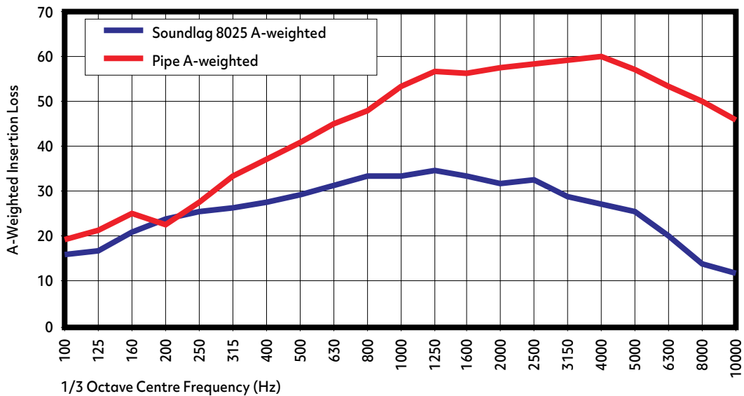
A- Weighted Insertion Loss of Bare Pipe versus pipe lagged with SOUNDLAG 8025
